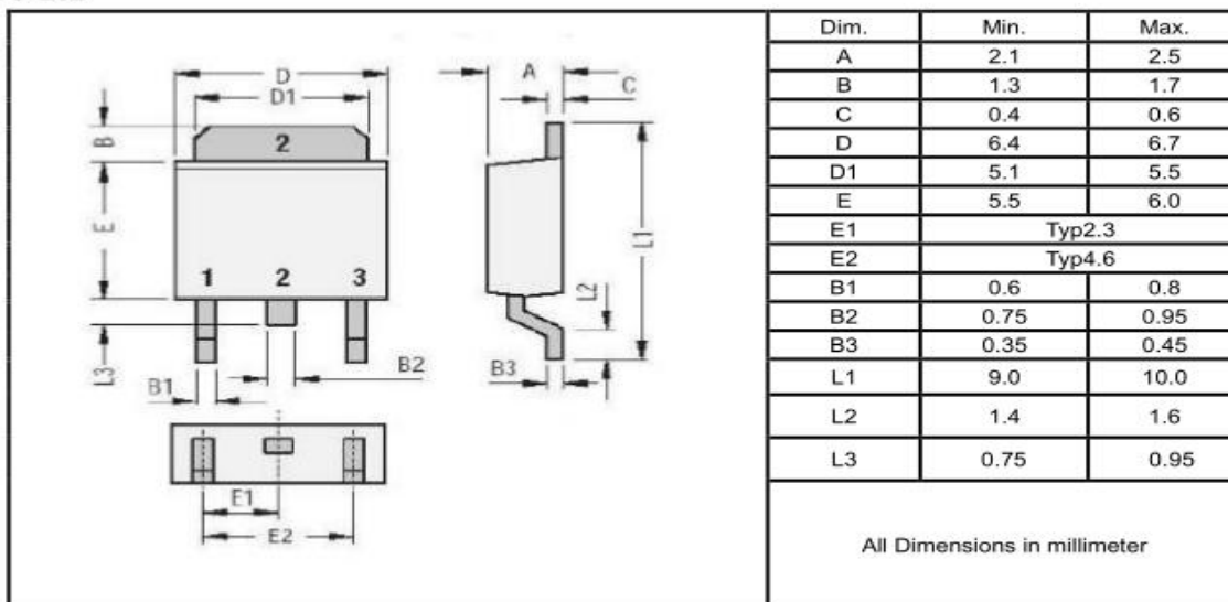
TO-252
