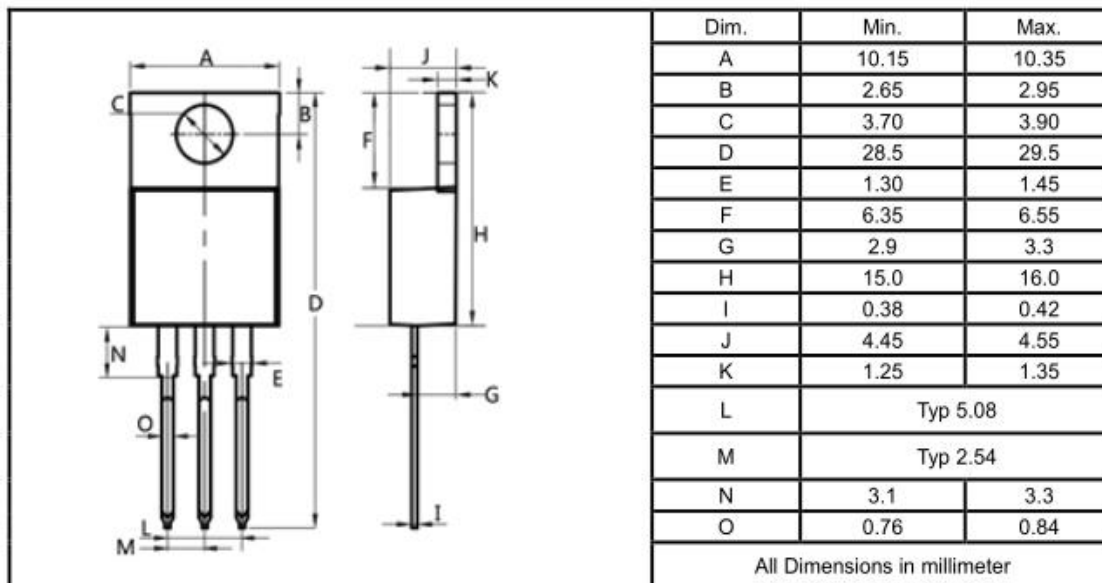
TO-220AB
