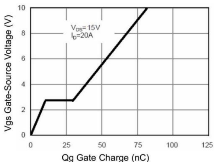
Figure 5 Gate Charge
