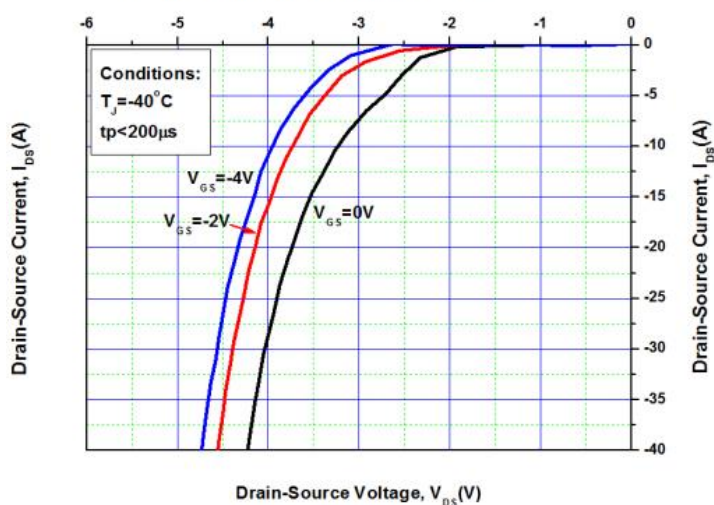
Figure 5. Body Diode Characteristic at -40^\circ\text{C}
