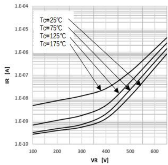
Figure 2 Reverse Characteristics
