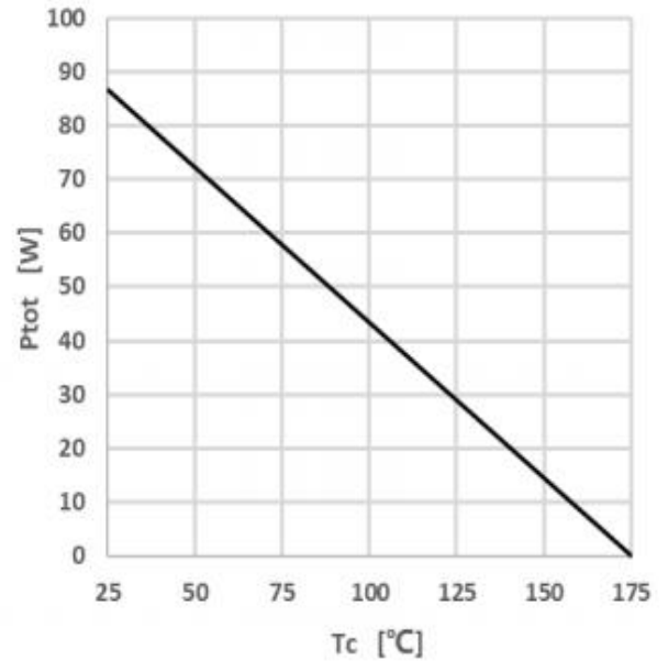
Figure 4 Power Dissipation
