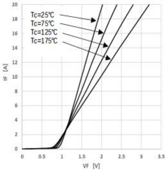
Figure 1 Forward Characteristics
