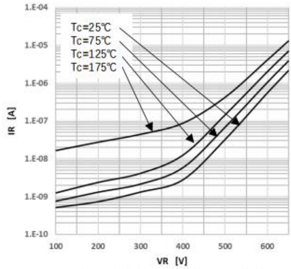
Figure 2 Reverse Characteristics
