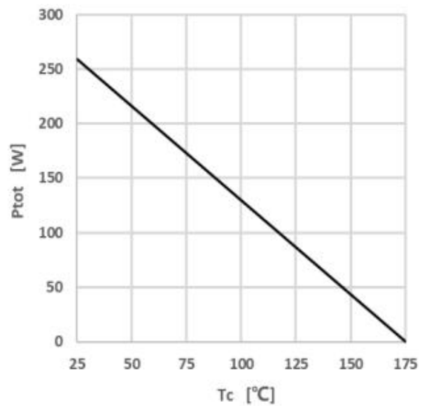
Figure 4 Power Dissipation
