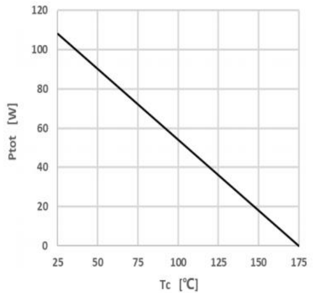
Figure 4 Power Dissipation
