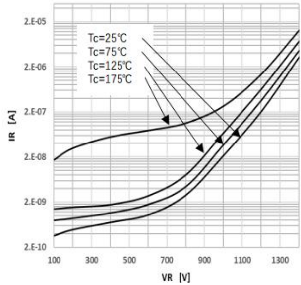
Figure 2 Reverse Characteristics
