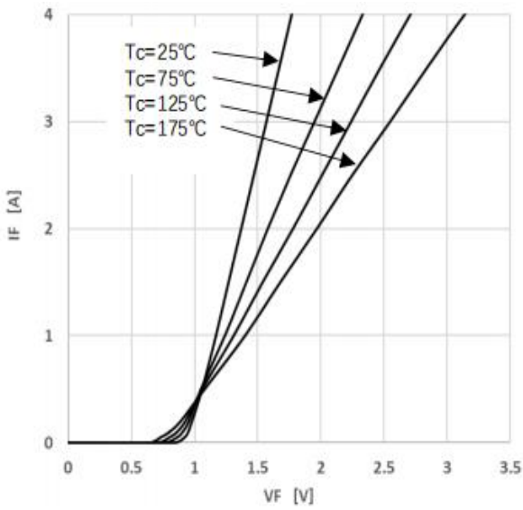
Figure 1 Forward Characteristics
