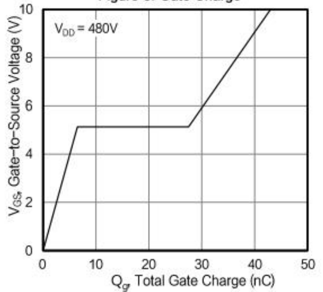
Figure 8. Gate Charge
