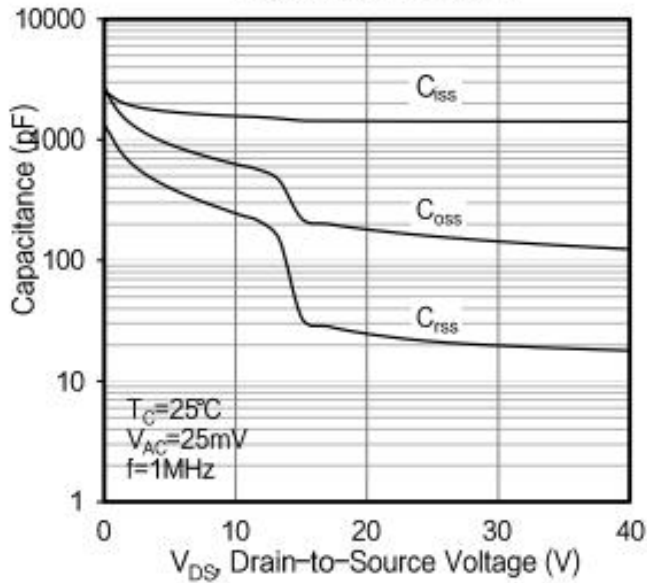
Figure 7. Capacitance
