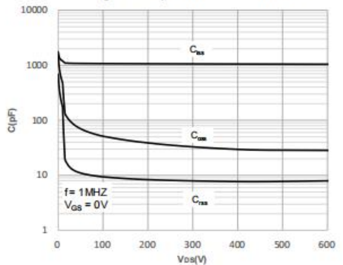
Figure 6: Capacitance Characteristics
