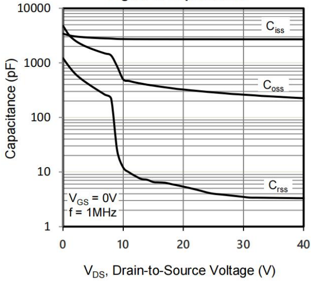
Figure 7. Capacitance
