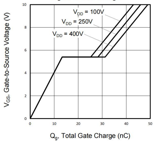
Figure 8. Gate Charge
