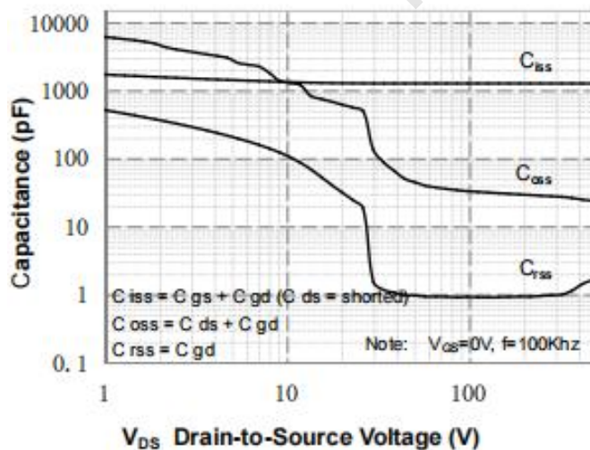
Figure 5. Capacitance Characteristics
