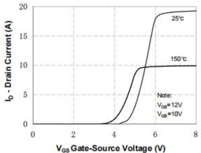
Figure 2. Transfer Characteristics vs Temperature
