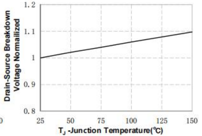
Figure 8. Drain-Source Breakdown Voltage vs Temperature
