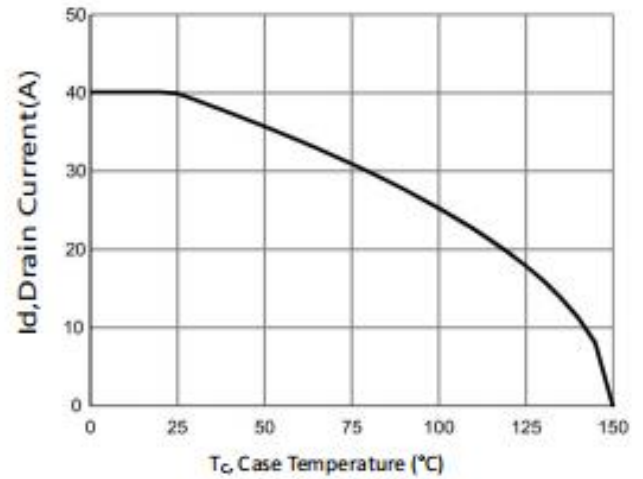
Figure10. Maximum Continuous Drain Current versus Case Temperature
