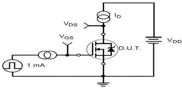
Gate Charge Test Circuit
