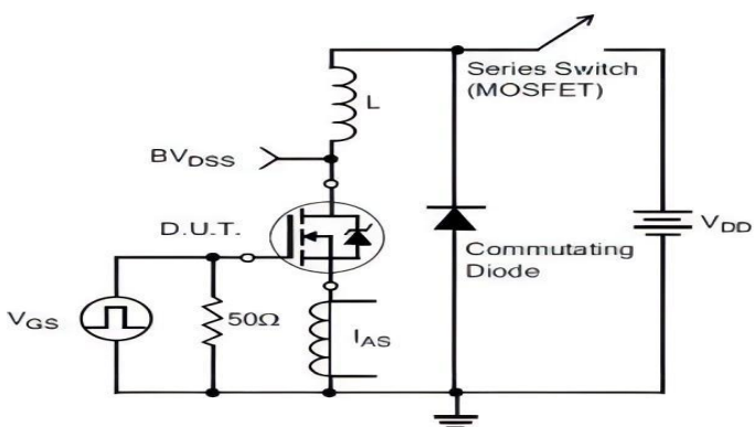
Unclamped Inductive Switching Test Circuit
