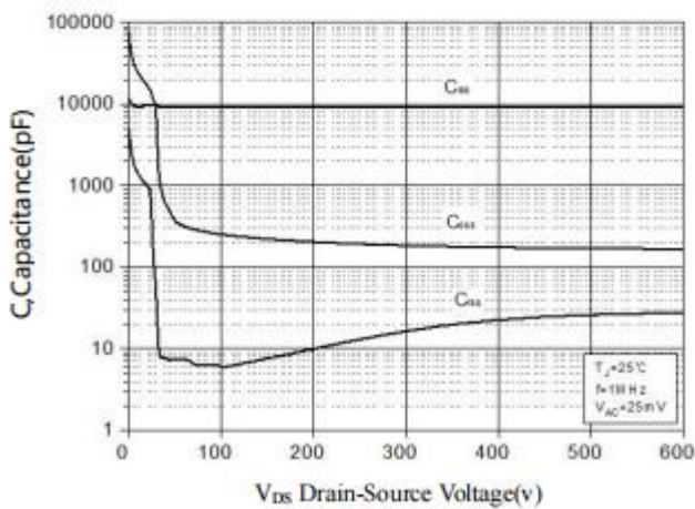
Figure5. Typical Capacitance versus VDS
