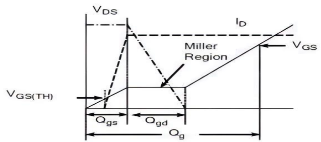
Gate Charge Waveform
