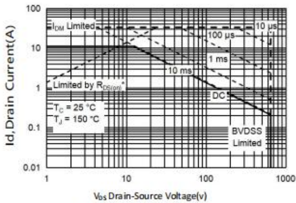
Figure9. Maximum Safe Operating Area TO-252
