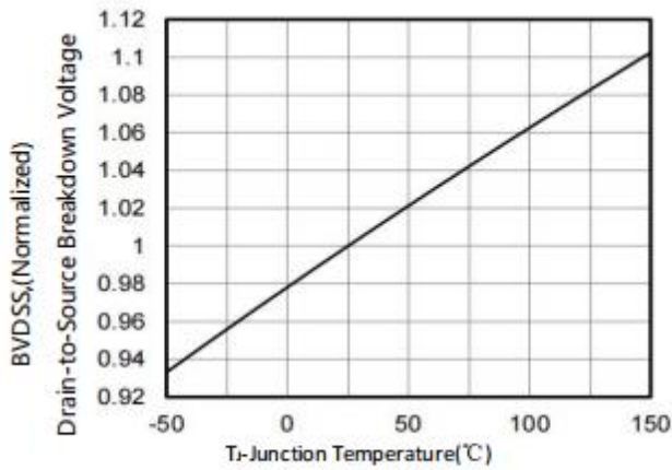
Figure7. BV_{DS} Variation with Temperature
