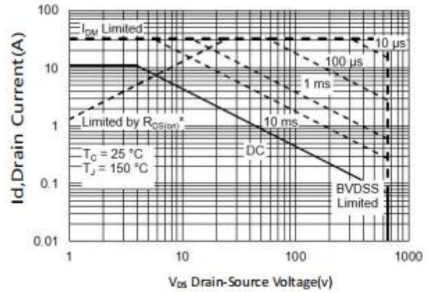
Figure9. Maximum Safe Operating Area TO-220F
