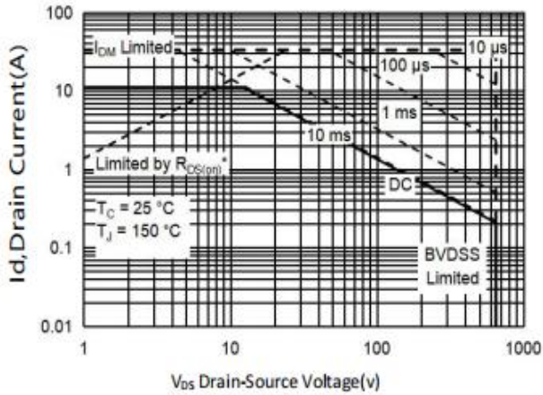
Figure9. Maximum Safe Operating Area TO-252
