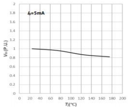
Fig6. Normalized Threshold Voltage vs. Temperature
